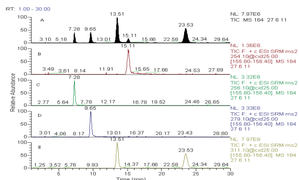
Figure 2: Total and extracted - ion chromatogram of the sulfonamides of 10 \mu\text{g/ml} at 0.4ml/min using 75:25 of formic acid and acetonitrile in isocratic mobile phase mode.
