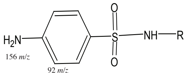
Figure 3: Scheme showing product ion formation for the sulfonamides following TSQ MS/MS fragmentation.
