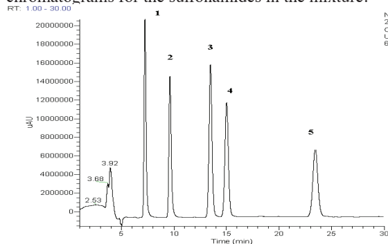
Figure 1: UV chromatogram (280nm) of injected sulfonamides solution at 10 \mu\text{g/ml} at 0.4ml/min using formic acid and acetonitrile (75:25 of 0.1% v/v) in as an isocratic mobile phase.
