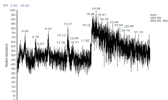
Figure 5: Total ion current 1mg/ml of propolis sample spiked with 50ng of STZ, SMZ, SDX, SMXZ, and SDMX using LTQ Orbitrap
