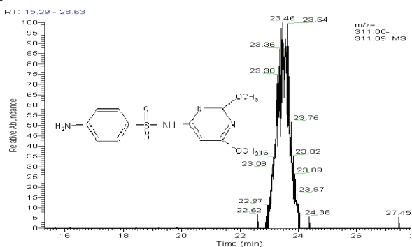
Figure 6: Sulfonamides in a 1 mg/ml of a propolis spiked sample with 50 ng of sulfonamides using LTQ Orbitrap spectrometer with restricted mass range for each compound, (A) STZ, (B) SMXZ, (C) SMZ, (D) SDX and (E) SDM X respectively.
