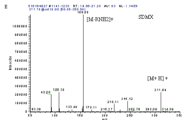
Figure 4: The ESI MS/MS full spectra show the identified protonated molecular ions [M+H]^+ and product ions of sulfonamides; (A) STZ, (B) SMZ, (C) SDX, (D) SMXZ, and (E) SDMX respectively.
