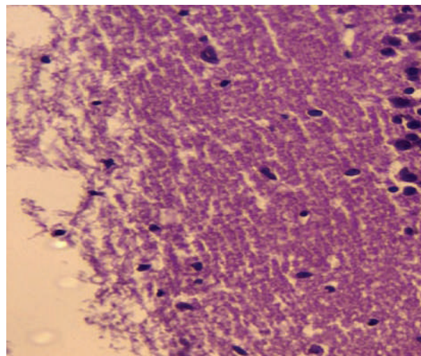
Fig. 5, A photomicrograph of group 1, control mouse brain treated with 1% T80, showing: unremarkable hippocampus (H&E. 40X).
