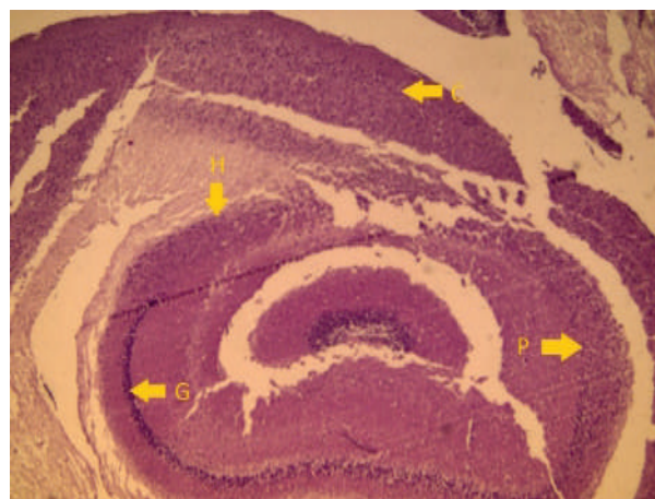
Fig. 1, A photomicrograph of group 1, control mouse brain injected with 1% T80, showing: normal histological structure for brain parts, cerebral cortex (C), and hippocampus (H) which shows normal granular (G) and pyramidal (P) layers. (H&E. 4X).
