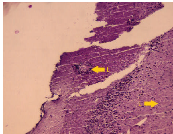
Fig. 6, A photomicrograph of group 2, mouse brain cerebral cortex, injected with scopolamine HBr 6 mg/kg, showing: mild cellular (lymphocytic) (L) infiltration and perivascular (L) aggregation. (H&E. X10).
