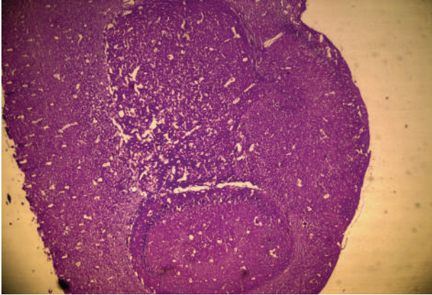
Fig. 18, A photomicrograph of group 5, mouse brain treated with scopolamine HBr followed by vitamin C, showed: vascular proliferation and edema in the cerebral cortex and hippocampus (H&E. X2.5)
