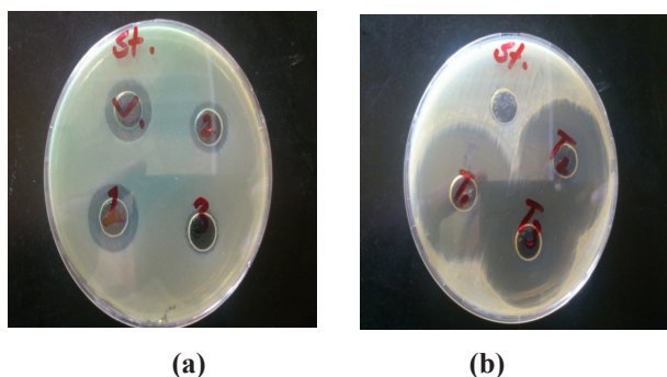
Figure 1: The effect of Penicillin G on S. aureus in the presence of Vitamin C 10 mg.
