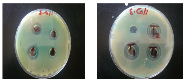
Figure 2: The effect of Penicillin G on E. coli in the presence of Vitamin C 10 mg.
