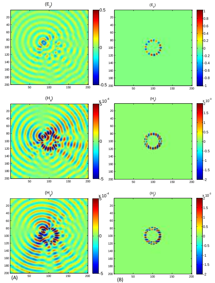
Fig.14. The TM z wave, electric field component (V/m) and magnetic components (A/m) generated at 250 time step: (A) inside the ring-shaped structure filled with a dielectric and (B) the dielectric surrounded by the PECs.
