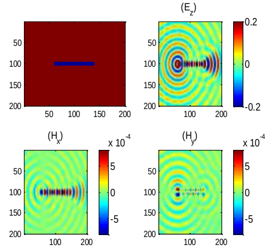
Fig.7. The TM_z wave, the electric field component (V/m) and magnetic fields (A/m) propagated inside the dielectric in the x direction.
