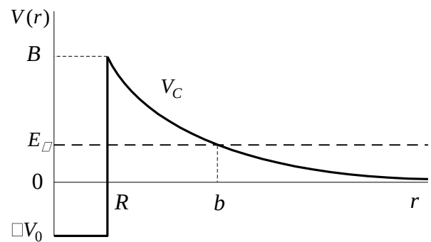
Fig.2. Nuclear potential well and the Coulomb potential V_C .
