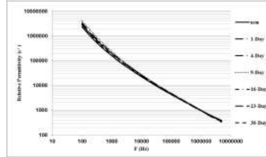
Fig.4. (a) Relative permittivity of brain tissues as a function of frequency (Hz) for grouped separately by time post-irradiation for single doses 4 Gy
