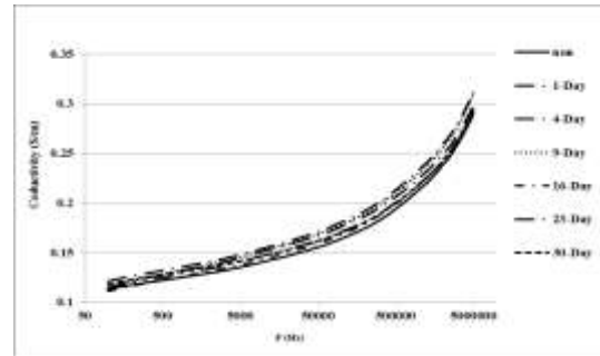
Fig. 2. (a) Conductivity (S/ m) of brain tissues as a function of frequency (Hz) for grouped separately by time post-irradiation for single doses 4 Gy
