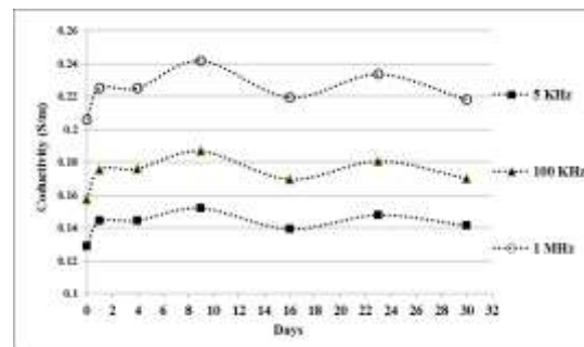
Fig. 3. Conductivity (S/ m) of brain as a function of time post-irradiation (days). The curves at low (5 KHz), intermediate (100 KHz) and high frequency (1 MHz)
