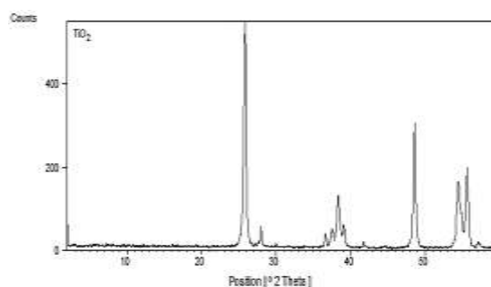
Fig. 6. XRD of nano titanium dioxide
