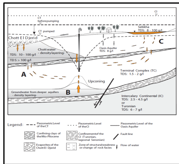
Figure 11. Conceptualization of the three differing salinization processes. A: Infiltration of brine from Chott; B: Upcoming of IC/Turonian water; C: Pollution by agricultural drainage water After [10].
