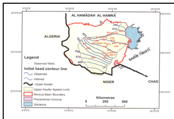
Figure 7. A map showing the general trend of groundwater movement towards the northeast of Murzuq Basin. After (El-Baruni & El-Futaisi, 2012)
