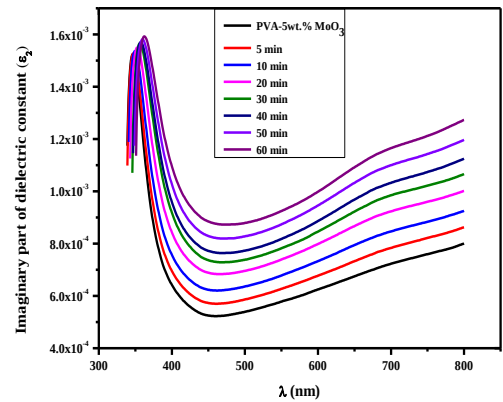
Fig.7. The imaginary constant of PVA-5wt. % MoO 3 film as a function of wavelength before and after UV irradiation.
