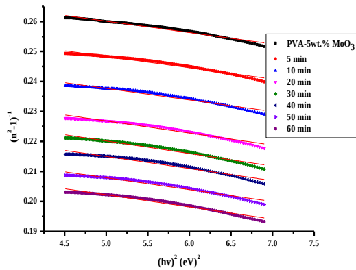
Fig.5. The relationship between (n^2-1)^{-1} and (hv)^2 for PVA-5wt. % MoO 3 film before and after UV irradiation.
