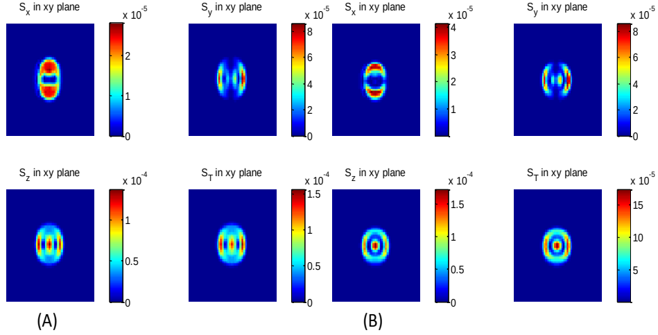
Figure 4. Images in the z plane which demonstrate the S_x , S_y , S_z and S_T . Three sources located in three locations: two cells apart (A) and source 1 placed overlapped with middle (B).
