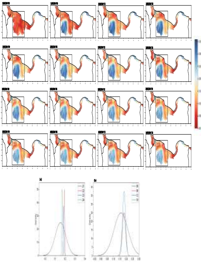
Fig.12. Volumetric soil moisture \text{m}^3 \cdot \text{m}^{-3} , for the 21 th at 00 hour to the 24 th at 18 hour at 2024
