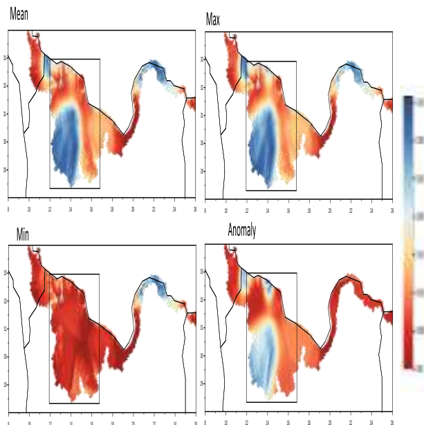
Fig.13. Volumetric soil moisture \text{m}^3 \cdot \text{m}^{-3} , Mean, Max, Min, Anomaly, for the 21 th at 00 hour to the 24 th at 18 hour at 2024
