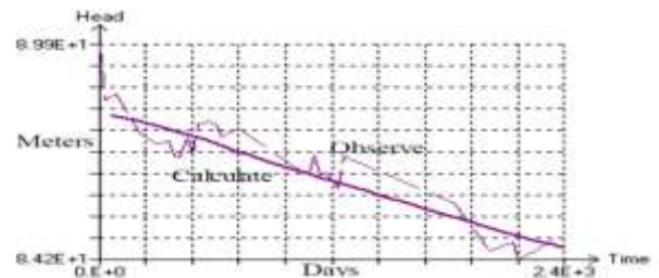
Fig. 16. Hydrograph Response of PZ57
