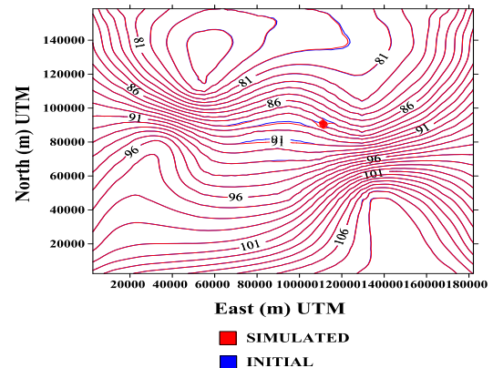
Fig .9. Steady Simulated Head (m.a.m.s.l) of the Surface (Shallow) Aquifer (1st)
