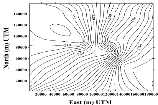
Fig. 8. Bottom of 2 nd producing) model layer (mams1)
