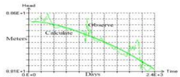
Fig.18. Hydrograph Response of PZ62
