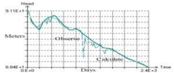
Fig. 15. Hydrograph Response of PZ55
