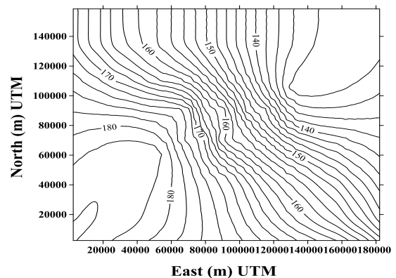
Fig. 7. Top of 2 nd (producing model layers) (mams)
