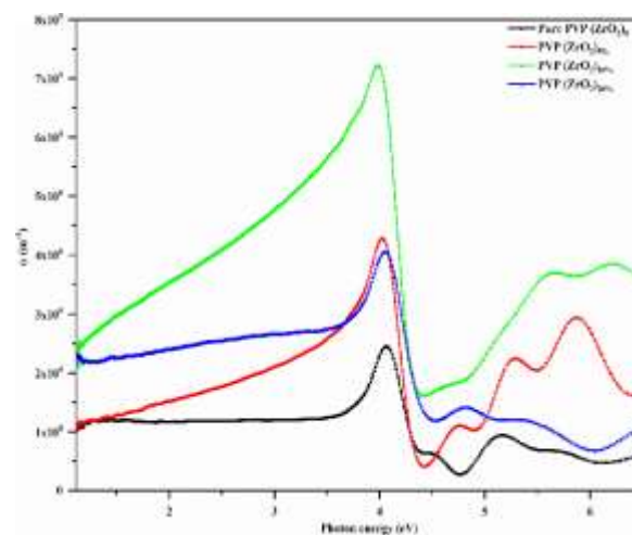
Fig. 7. Optical absorption coefficient versus photons energy for PVP pure and doped with different % \text{ZrO}_2
