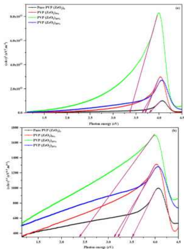
Fig.9. Direct (a) and indirect (b) optical band gap energies for PVP pure, and doped with different % \text{ZrO}_2
