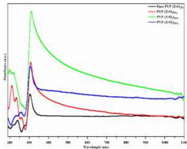
Fig.6. UV-Visible absorption spectra of PVP pure, and doped with different % \text{ZrO}_2
