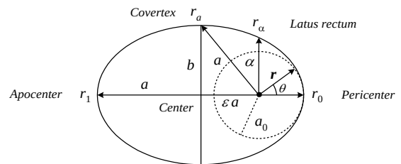
Figure 1. Common parameters used to describe elliptical orbits.
