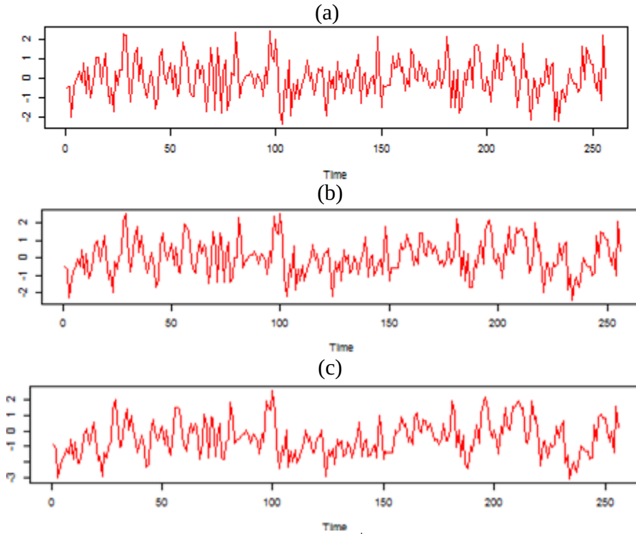
Fig. 3. Simulated time series for ARFIMA(0, d^* , 0) processes with fixed sample size 256 and different values of d^* (a) d^* = 0.1 , (b) d^* = 0.3 and (c) d^* = 0.45 .
