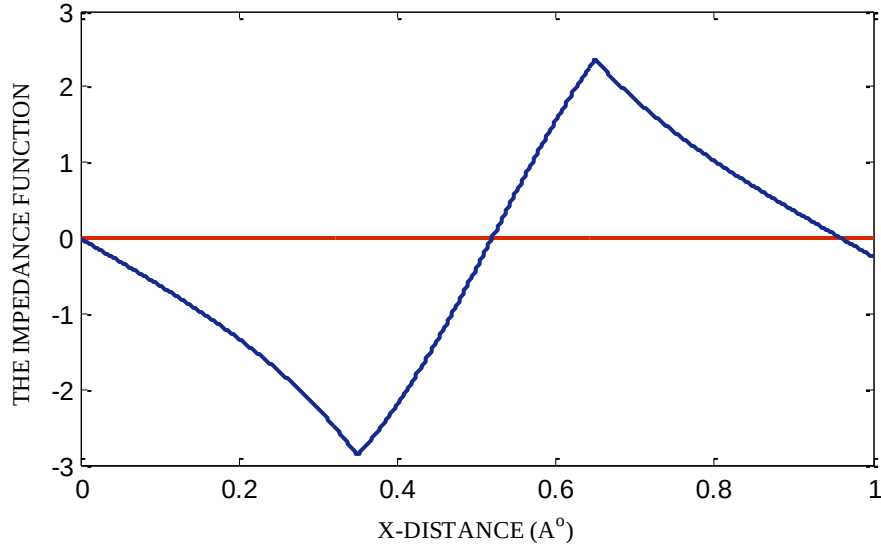
Figure 1. The impedance function for an electron in a unit cell with a=1 \text{ A}^0 having a central square well potential with b=0.3 \text{ A}^0 and V_0=100 \text{ eV} at energy eigenvalue E=23.179 \text{ eV} .
