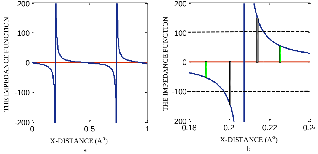
Figure 2a. The impedance function for an electron in a unit cell with a = 1 \text{ Å} having a central square well potential with b = 0.3 \text{ Å} and V_0 = 100 \text{ eV} at energy eigenvalue E = 218.781 \text{ eV} .
