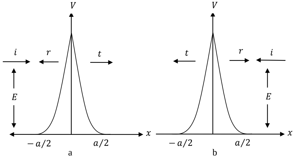
Figure 6. An arbitrary symmetric potential extending from -a/2 to a/2 .
