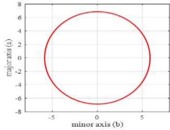
Fig. 7. Spherical shape for ^{138}\text{Ba} isotope
