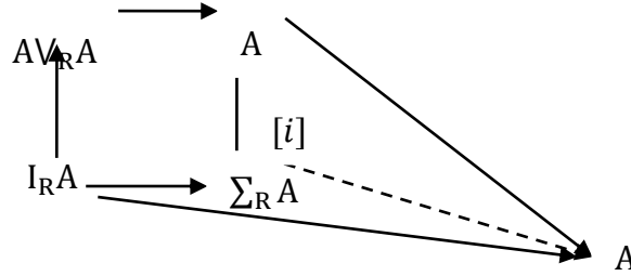
Figure 1: torus \sum_R A
