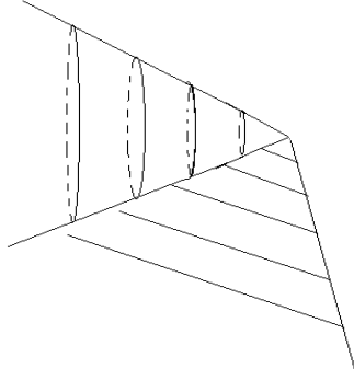
Figure 3. (\Sigma(R \sqcup R))_{\text{Glue}}
