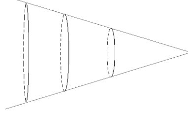
Figure 4. (\sum(R \sqcup R))_{\text{Glue}} \simeq (R \sqcup R)^2
