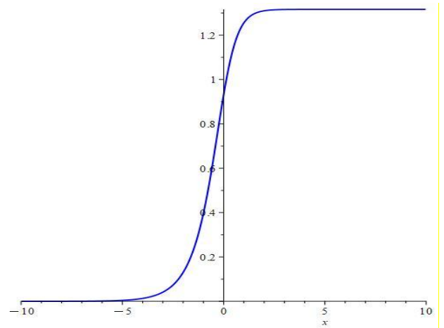
Figure 1. The profile of the dark-soliton solution (3.7) with
