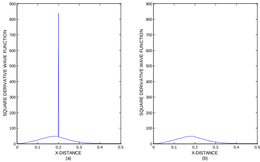
Figure 3. a) The square derivative of wave function and b) singularity removed.
