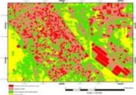
b-Classified Landsat 2006
