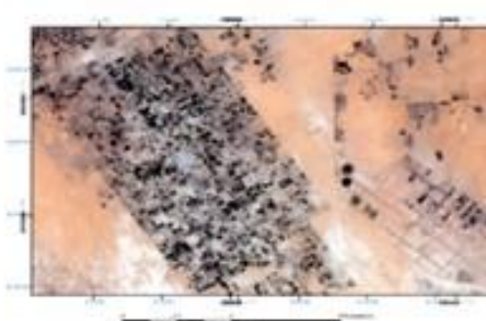
a-Sentinel-2 Image-2022
