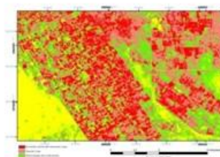
b-Classified Sentinel-2- 2018
