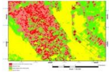
b-Classified Sentinel-2 - 2022
