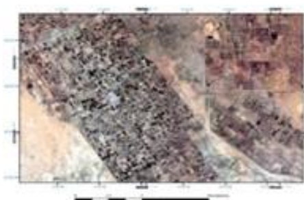
a- Sentinel-2 Image-2018
