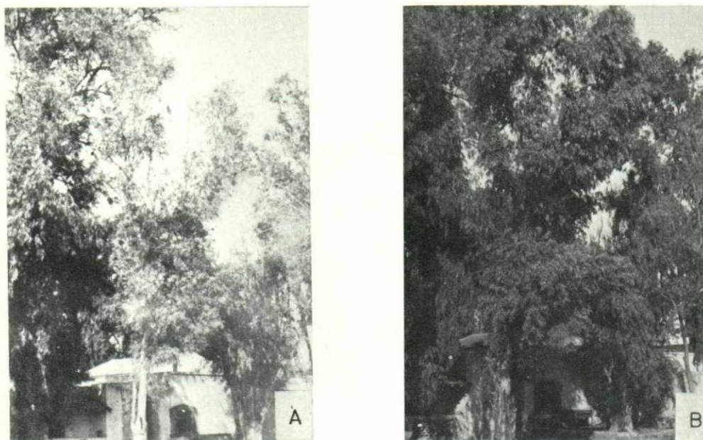
Fig. 1. (A & B). Eucalyptus tree, before and 60 days after injection with iron citrate, respectively.
