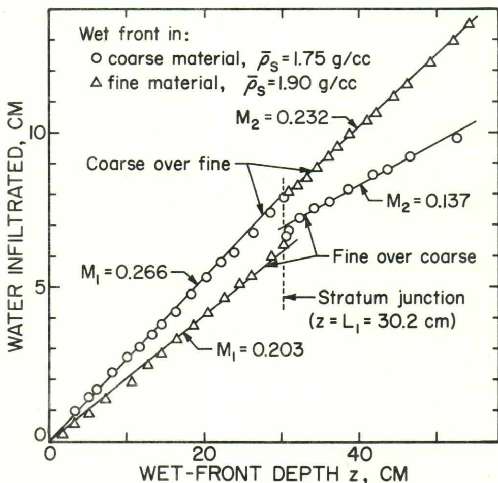
Fig. 1. Water infiltrated versus wet-front advance, for stratified columns of coarse over fine and fine over coarse, with depth of upper stratum L_1 = 30.2 cm in both instances.
