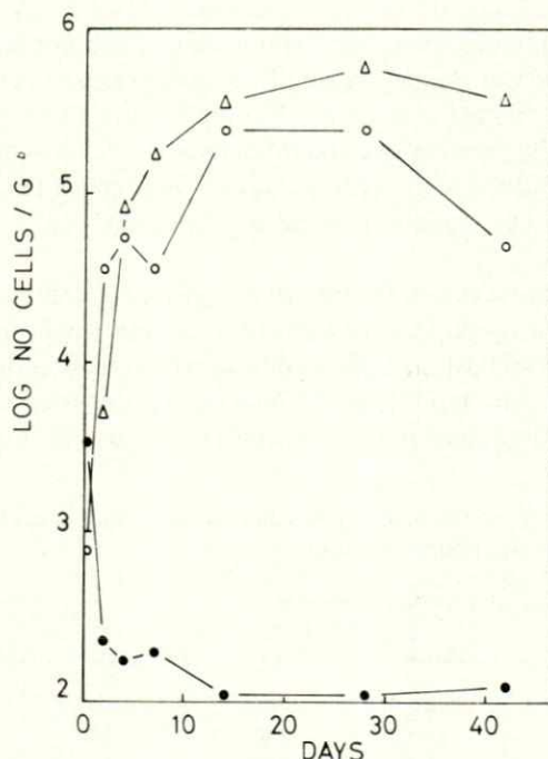
Fig. 1. Growth of Nitrosomonas spp. in incubated soils treated with ammonium sulphate alone (Δ) or in combination with dextrose (○) or casein (●). (b) 95% confidence interval was D/3.30 to 3.30 D where D is the number of bacteria.
