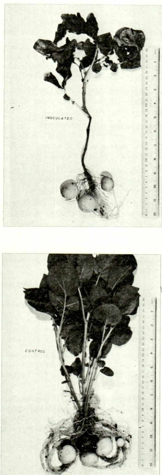
Fig. 1. Healthy (control) and infected potato plants after artificial inoculation.
