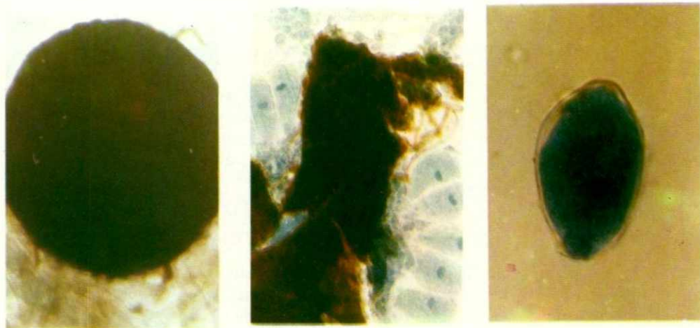
Fig. 3. Erysiphe graminis from Bromus diandrus . A. A peritheciium with rudimentary appendages and hyaline bristles; B. A ruptured peritheciium with several asci without ascospores; C. A single ascus without ascospores.
