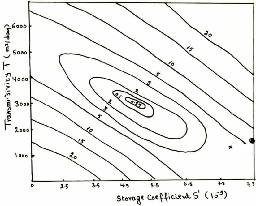
Fig. 6. Contours of the objective function (O) of El-Nybaria pumping test, Well No. 22. x Values of T and S' received by graphical method. O Values of T and S' received by computer method.
