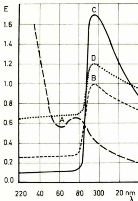
Fig. 3. UV-absorption spectra of: (A) The original samples of 'Rub Al-Tamr', (B) The filtrate after treatment with charcoal, (C) The colouring matters adsorbed on charcoal, (D) The filtrate after treatment with alcohol.
