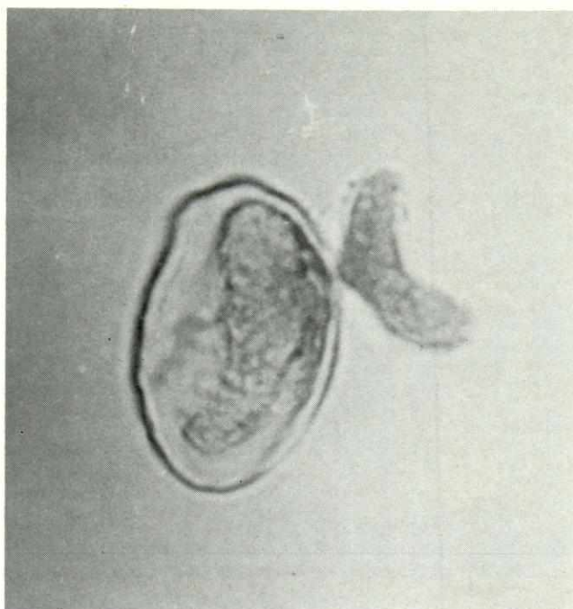
Fig. 3. Conidium of Sphaerotheca fuliginea from cucumber showing forked germ tube.
