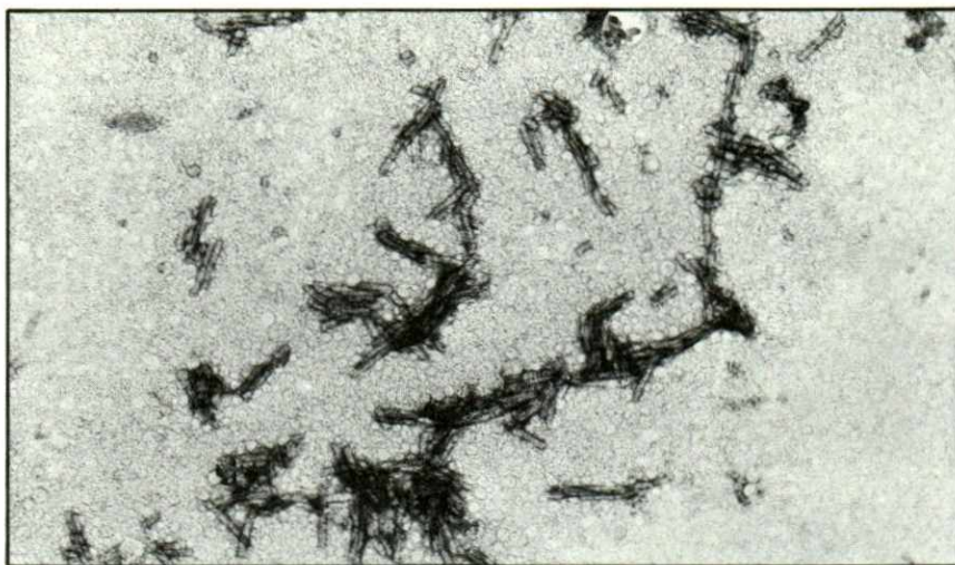
Fig. 3 An electron micrograph of the potato virus isolate negatively stained with 2% uranyl acetate showing slightly flexuous broken particles (X 70,000).
