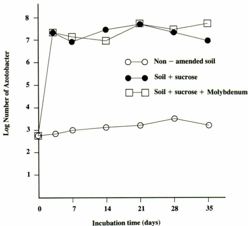
Fig. 2 Estimated most-probable number of Azotobacter in soil as influenced by sucrose addition (1%) with and without molybdenum (5ppm). (b) 95% confidence interval was D/3.3 to 3.3D , where D is the number of cells.
