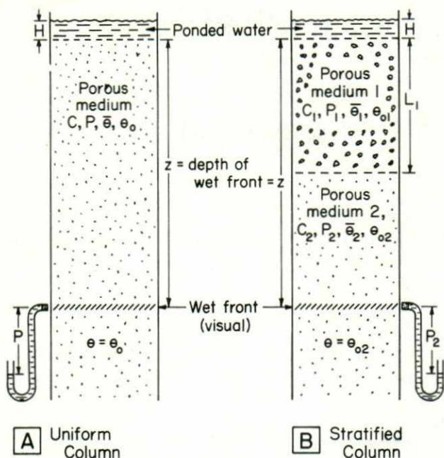
Fig. 1. Diagrams of water infiltration into columns of porous media, (A) a uniform column, and (B) a stratified column.
