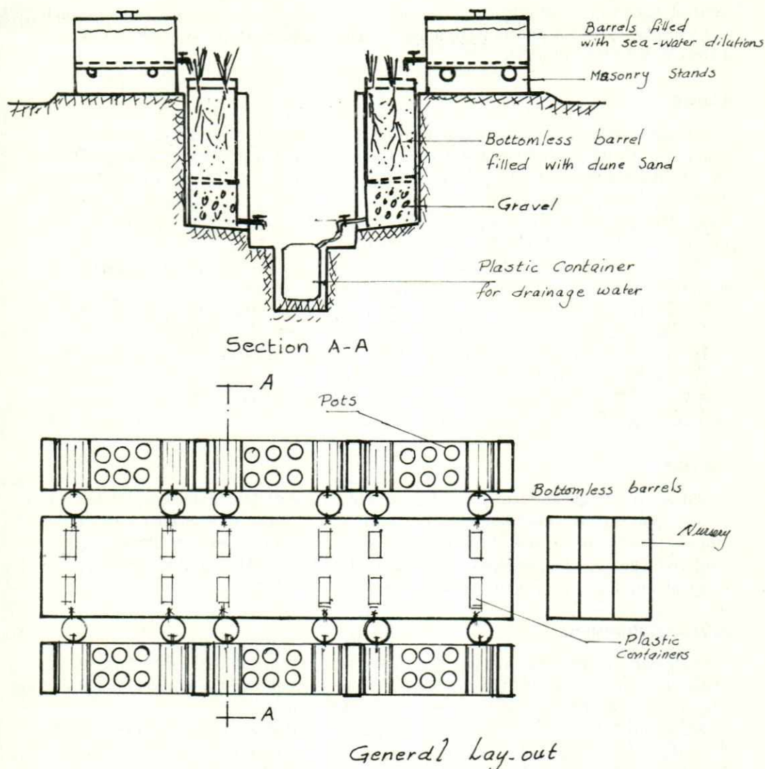
Fig. 1. Schematic plan and cross section for the experiment.
