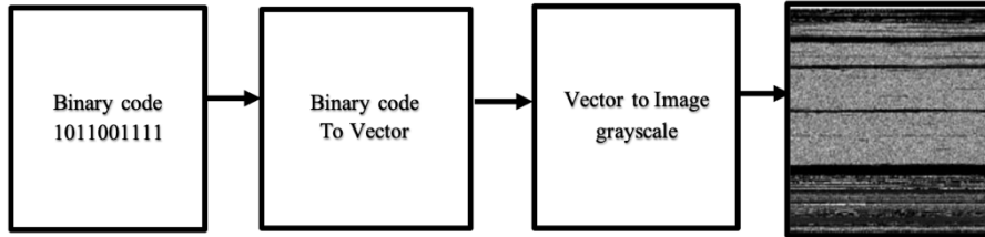
Fig. 6. Representation of Malware as an Image
